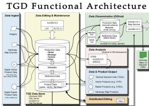
Figure 1. TGD Functional Architecture
